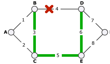
Figure 1. Example network in which link 4 is protected by path 3–5–6.
