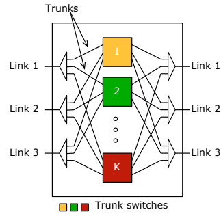
Figure 5. Node architecture in a Trunk Switched Network.
