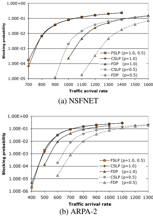
Figure 8. Blocking probability in the NSFNET and ARPA-2 networks.
