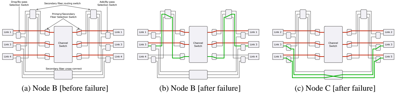
Figure 2. Switch settings at nodes under FSLP approach before and after link 4 failure.
