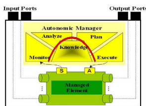
Figure 1: Autonomic Component Model
